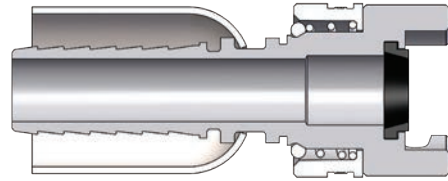
Dual-Lock P-Series Coupler with Ferrule (Hose Barb)
