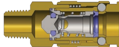
CJ-Series European Interchange Coupler (Male Threads)
