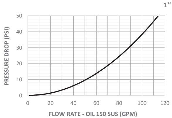
Rated Pressure Chart
