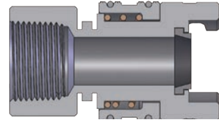
Dual-Lock P-Series Coupler (Female Threads)
