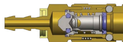
U-Series Automatic Universal Coupler (Push-Loc Barb)
