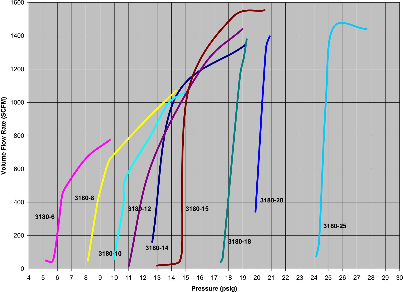
3180 Pressure Relief Valve - Flow Rate Vs Pressure
